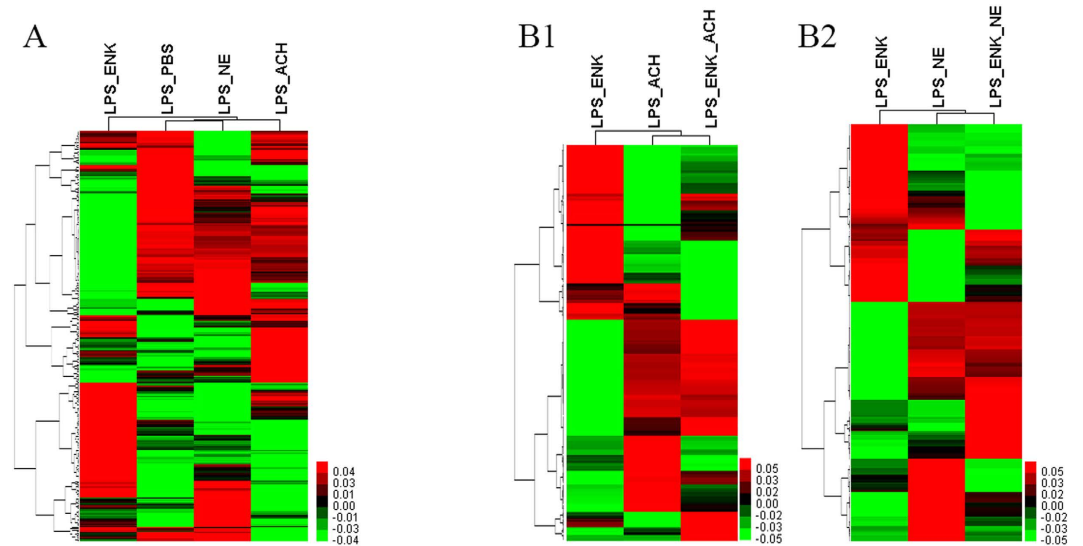
Figure 4. Cluster map of differentially expressed immune-related genes. (A) Summary cluster map of differentially expressed immune-related genes among the gene lists of LPS_ENK, LPS_ACh and LPS_NE. (B1) Summary cluster map of differentially expressed immune-related genes among the gene lists of LPS_ENK, LPS_ACh and LPS_ENK_ACh. (B2) Summary cluster map of differentially expressed immune-related genes among the gene lists of LPS_ENK, LPS_NE and LPS_ENK_NE.
