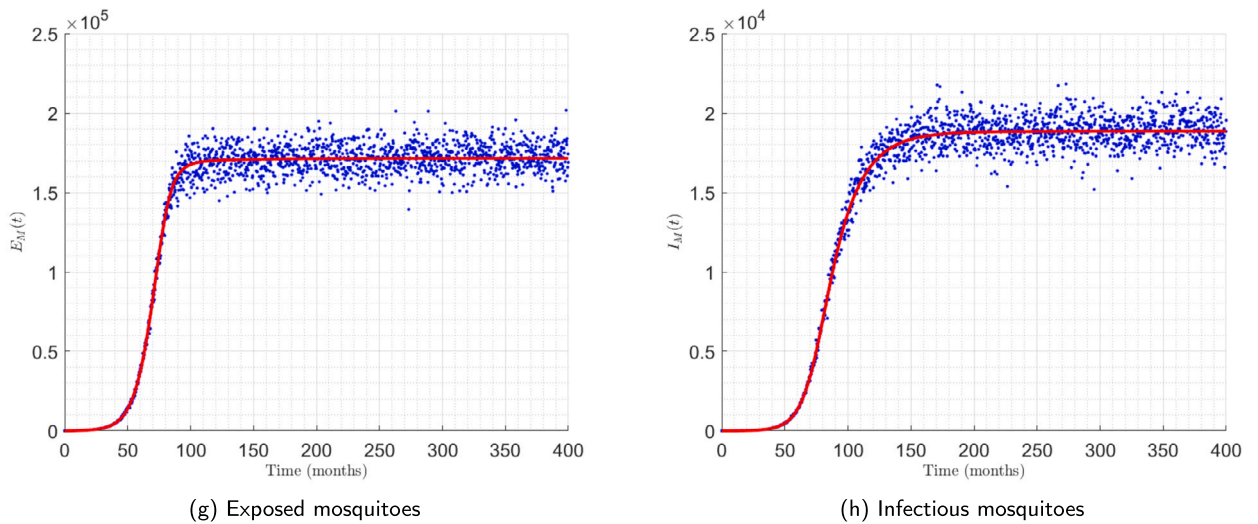
Fig. 6. Scatter estimated with standard deviation of 0.05 and numerical simulation (sold) with confidence interval of 95%.
