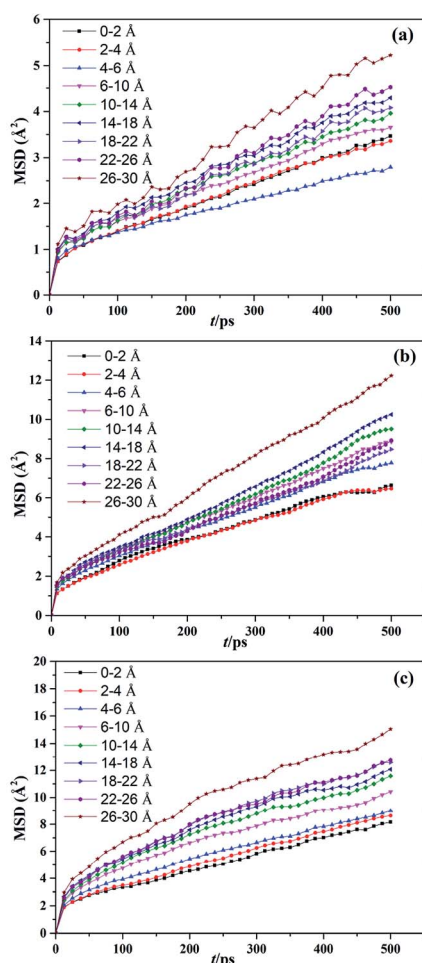
Fig. 7 MSDs of the silica/g10 composite at different temperatures of (a) 200, (b) 298, and (c) 373 K.
