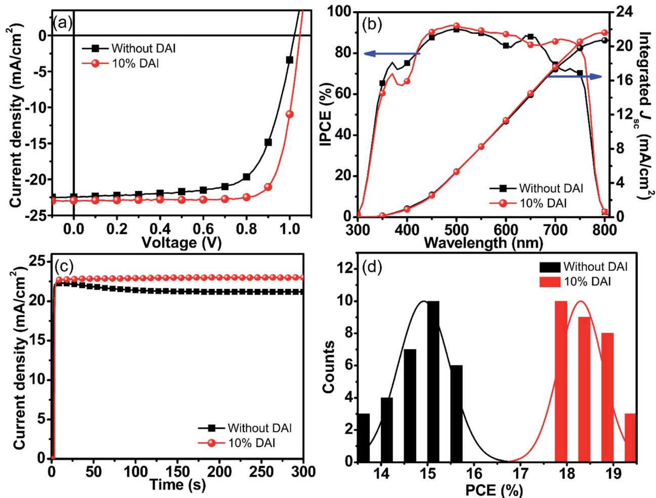
Fig. 4 J - V characteristics (a), EQE spectra (b), stabilized short-circuit photocurrent density (c), and PCE distribution (d) of the perovskite devices without and with 10% DAI contents.
