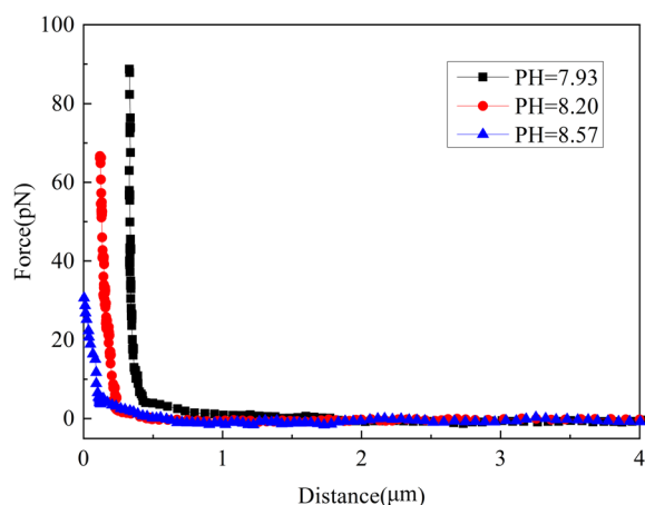
Fig. 9 Force–distance curve in the alkaline solutions.
