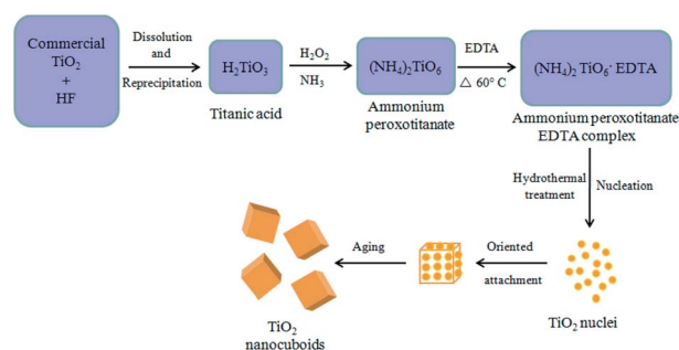
Fig. 7 A proposed mechanism for the formation of \text{TiO}_2 nanocuboids.
