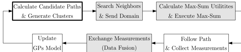
Figure 4. Algorithm block diagram. Shaded blocks represent modules that require communication between robots.
