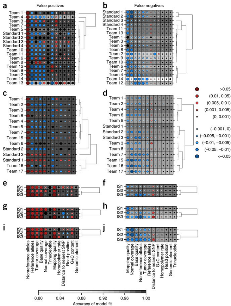
Figure 5. Characteristics of prediction errors. (a–j) Random Forests assess the importance of 12 genomic variables on SNV prediction accuracy (Online Methods). Random Forest analysis of FPs (a,c,e,g,i) and FNs (b,d,f,h,j) for IS1 (a,b) and IS2 (c,d) as well as for all three tumors using default settings with widely used algorithms MuTect (e,f), SomaticSniper (g,h) and Strelka (i,j). Dot size reflects mean change in accuracy caused by removing this variable from the model. Color reflects the directional effect of each variable (red for increasing metric values associated with increased error; blue for decreasing values associated with increased error; black for factors). Background shading indicates the accuracy of the model fit (see bar at bottom for scale). Each row represents a single set of predictions for a given in silico tumor, and each column shows a genomic variable. SNP, single-nucleotide polymorphism.
