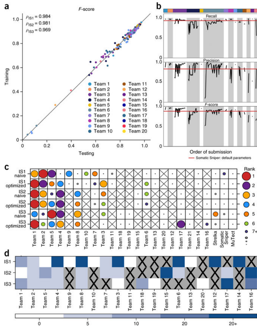
Figure 3. Effects of algorithm tuning. (a) The performance of groups on the training data set and on the held-out portion of the genome (~10%) are tightly correlated (Spearman’s \rho = 0.98 ) and fall near the plotted y = x line for all three tumors. (b) F -score, precision and recall of all submissions made by each team on IS1 are plotted in the order they were submitted. Teams were ranked by the F -score of their best submissions. Color coding as in a . The horizontal red lines give the F -score, precision and recall of the best-scoring algorithm submitted by the Challenge administrators, SomaticSniper. A clear improvement in recall, precision and F -score can be seen as participants adjusted parameters over the course of the challenge. Bar width corresponds to the number of submissions made by each team. (c) For each tumor, each team’s initial (“naive”) and final (“optimized”) submissions are shown, with dot size and color indicating overall ranking within these two groups. An “X” indicates that a team did not submit to a specific tumor (or changed the team name). Algorithm rankings were moderately changed by parameterization. (d) For each tumor, we assessed how much each
