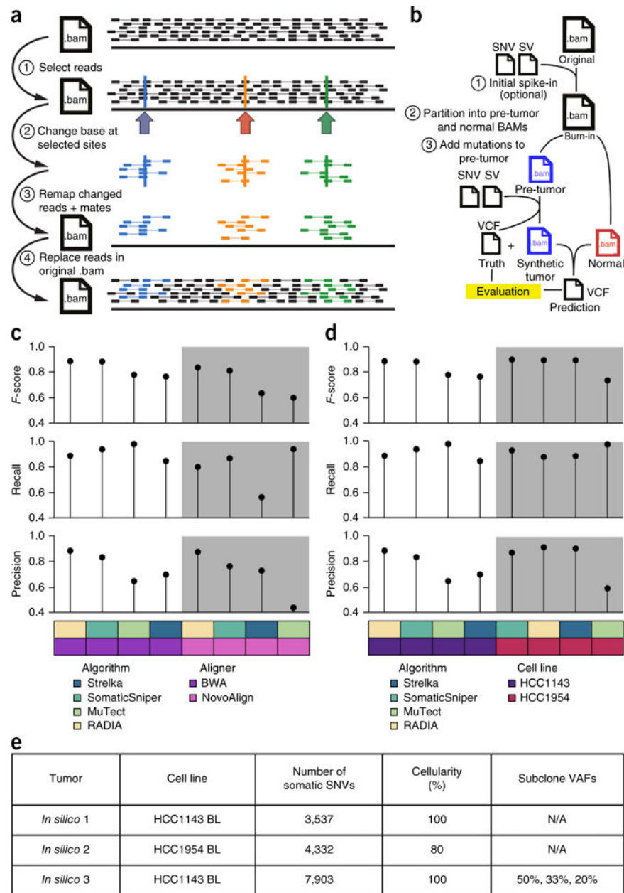
Figure 1. BAMSurgeon simulates tumor genome sequences. (a) Overview of SNV spike-in. (1) A list of positions is selected in a BAM alignment. (2) The desired base change is made at a user-specified variant allele fraction (VAF) in reads overlapping the chosen positions. (3) Altered reads are remapped to the reference genome. (4) Realigned reads replace corresponding unmodified reads in the original BAM. (b) Overview of workflow for creating synthetic tumor-normal pairs. Starting with a high-depth mate-pair BAM alignment, SNVs and structural variants (SVs) are spiked in to yield a ‘burn-in’ BAM. Paired reads from this BAM are randomly partitioned into a normal BAM and a pre-tumor BAM that receives spike-ins via BAMSurgeon to yield the synthetic tumor and a ‘truth’ VCF file containing spiked-in positions. Mutation predictions are evaluated against this ground truth. (c,d) To test the
