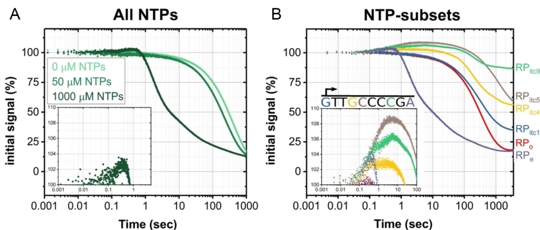
Figure 4. Transient peak signal present at high NTP concentrations is due to initial transcribing complexes. (A) Comparison of dissociation and promoter escape for Mtb. Mtb holo RP_o mixed with 25 \mu\text{g/ml} salmon-sperm DNA, 50 \mu\text{M} NTPs, and 1000 \mu\text{M} NTPs (concentrations following equal volume mixing). Inset shows the percent increase above the starting fluorescence signal plotted from 0.001 to 5 s. (B) NTP-subset experiments for Mtb. Mtb holo RP_o mixed with salmon-sperm DNA only ( RP_e , red) or with salmon-sperm DNA and initiating nucleotide (GTP, RP_{itc1} , blue), nucleotides sufficient for formation of a 4-mer (G/UTP, RP_{itc4} , yellow), nucleotides sufficient for formation of a 5-mer (G/UTP and 3'-O-methyl-CTP, RP_{itc5} , brown), nucleotides sufficient for formation of a 9-mer (G/U/CTP, RP_{itc9} , green) or all four nucleotides to allow escape ( RP_e , purple). NTP additions yielded a final concentration of 1000 \mu\text{M} for each NTP following equal volume mixing. Inset depicts peak signal plotted from 0.001 to 100 s with the initially transcribing sequence of the non-template strand listed above.
