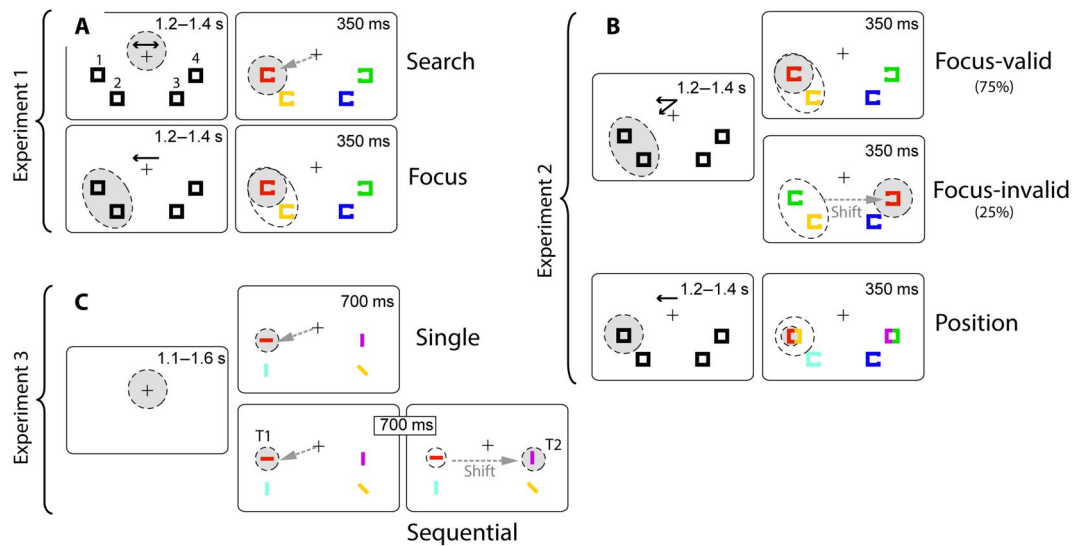
Fig. 1. Experimental design. In three experiments, participants performed different versions of a search task for a colored item, reporting its orientation (“C” site of gap; bars, vertical, diagonal, or horizontal) via button press. Gray circles illustrate the focus of spatial attention, and gray dashed arrows illustrate its shift. (A) Experiment 1. Permanent placeholders (black rectangles) demarcated positions of upcoming stimuli (1 to 4). Endogenous cues (black arrows) informed participants every 10 trials about the current experimental focusing condition. The cue could be uninformative (search condition) or point to the visual hemifield of the upcoming target (here, red C), allowing for prefocusing (focus condition). (B) Experiment 2. Focus condition as in experiment 1 (focus-valid), except that, on 25% of the trials, the target appeared in the uncued hemifield (focus-invalid). Position task (position): Target appeared at the indicated item position (one of four) together with a differently colored distractor item. At the mirror position, an analogous two-color distractor was shown. (C) Experiment 3. Similar to search condition of experiment 1 but without placeholders or uninformative cues. On half of the blocks, participants were instructed to report the orientation of the color-defined target (single). On the remaining trial blocks, they had to use the orientation direction of the color target (T1) to shift their attention to a second target (T2) and report its orientation (sequential). Note that the exact size and distance of the search items shown in the figure differ from how they were presented during the experiment.
