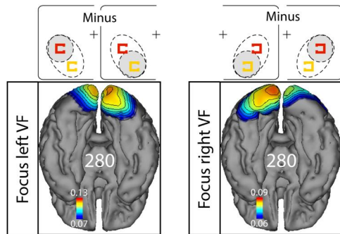
Fig. 4. Within-cued quadrant analysis (experiment 1). Left: Source estimates of the response difference elicited by a target in the top left minus the bottom right item position in the bottom left visual quadrant of the focus condition. Right: Response difference elicited by a target in the bottom left minus the top right item position in the bottom right visual quadrant.
