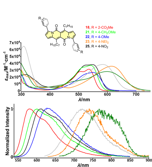
Fig. 4 Top: absorption spectra of compounds 18 (red), 21 (green), 22 (blue), 23 (orange) and 25 (black) measured in dichloromethane. Bottom: normalized emission spectra of compounds 18 (red), 21 (green), 22 (blue), 23 (orange) and 25 (black) measured in dichloromethane. Adapted with permission from ref. 30a. Copyright 2018 Wiley.
