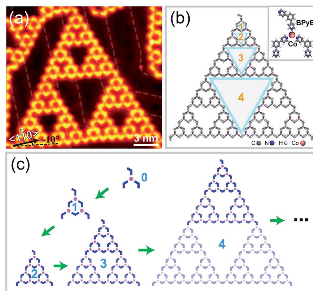
Fig. 1 Fractal phase formed at low molecular coverage. (a) STM image of a defect-free ST of 4 order; inset: coordinated trimer acting as basic recursive unit. The white arrow indicates \langle 1\bar{1}0 \rangle direction. Scanning parameters: constant-height mode, V_B = 10 mV, I_t = 80 pA. (b) Structural model of the ST in (a). (c) Schematic models revealing the evolution process of fractal phase.
