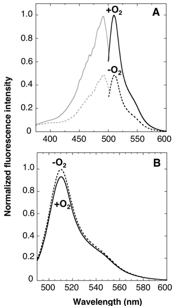
Figure 6. Spectroscopic properties of ANA-G. (A) Excitation (gray color) and emission (black color) spectra of ANA-green (ANA-G; 1 \mu\text{M} ) were measured in the absence (dashed line) or presence (solid line) of 240- \mu\text{M} oxygen. Excitation and emission spectra of ANA-G were measured at emission and excitation wavelengths of 510 and 490 nm, respectively. (B) Emission spectra of ANA-G His348Ala variant (1 \mu\text{M} ) in the absence (dashed line) or presence (solid line) of 240- \mu\text{M} oxygen; Data are presented relative to the fluorescence intensity of ANA-G in the presence of oxygen (1.0).
