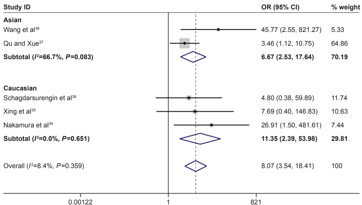
Figure 4 Forest plot for the association between Ras-associated domain family 1A promoter methylation and risk of papillary thyroid carcinoma. Abbreviations: CI, confidence interval; OR, odds ratio.
