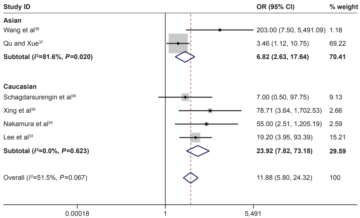
Figure 3 Forest plot for the association between Ras-associated domain family 1A promoter methylation and risk of follicular thyroid carcinoma. Abbreviations: CI, confidence interval; OR, odds ratio.
