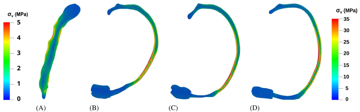
FIGURE 8 Von Mises stress distributions ( \sigma_v ) on selected slices for the case with a 600 N force applied at the compression region P2. In part (A), the slice corresponds to the saggital mid-plane along the breastbone, with the \sigma_v levels as shown in the leftmost colorbox. In parts (B–D), slices along the breastbone, costal cartilages and osseous ribs are respectively shown for the 3rd, 4th, and 5th left ribs, with the \sigma_v levels in the rightmost colorbox
