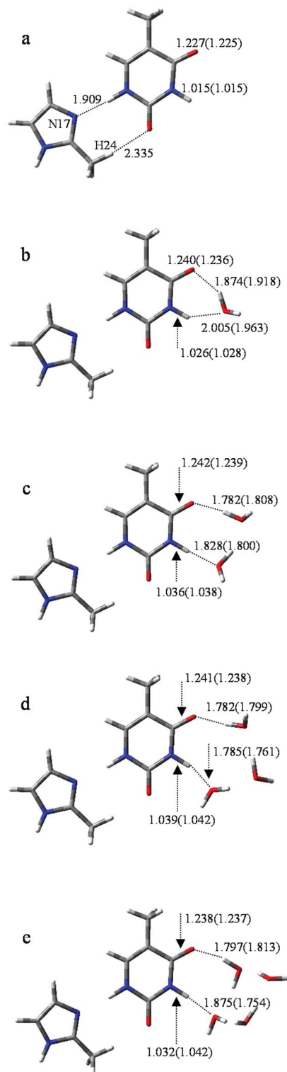
Fig. 3 Optimized geometries of T- nw combined with M. Data listed in parentheses is the bond distances ( \text{\AA} ) of T- nw .
