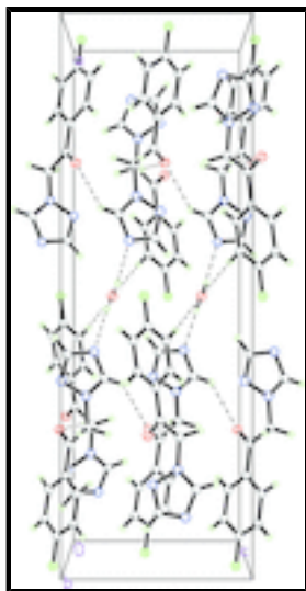
Fig. 2. A packing diagram of the title compound showing the intermolecular O—H...N hydrogen bonds (dashed lines).
