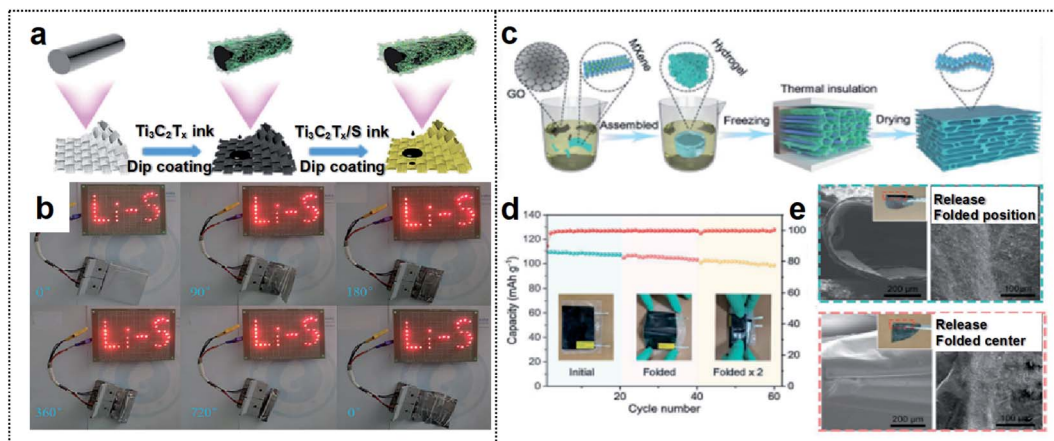
Fig. 5 MXene-based foldable 2D electrode. (a) Schematic illustration of the fabrication process of the MF@ \text{Ti}_3\text{C}_2\text{T}_x/\text{S} cathode. (b) A “Li–S” shaped string of light contains 30 LEDs lit by MF@ \text{Ti}_3\text{C}_2\text{T}_x/\text{S} 50 electrode soft-packaged Li–S batteries at different bending angles. Reproduced from ref. 82. Copyright 2021, Royal Society of Chemistry. (c) Schematic illustration of the fabrication process of the MGA material. (d) Cycling performance of the LMO//MGA@Zn pouch cells at various folding times. (e) SEM images of the MGA sample after folding (left) and releasing (right) once (up) and twice (down). The inset images indicate the optical pictures of the MGA sample after folding once (up) and twice (down), respectively. Reproduced from ref. 83. Copyright 2021, Wiley-VCH.
