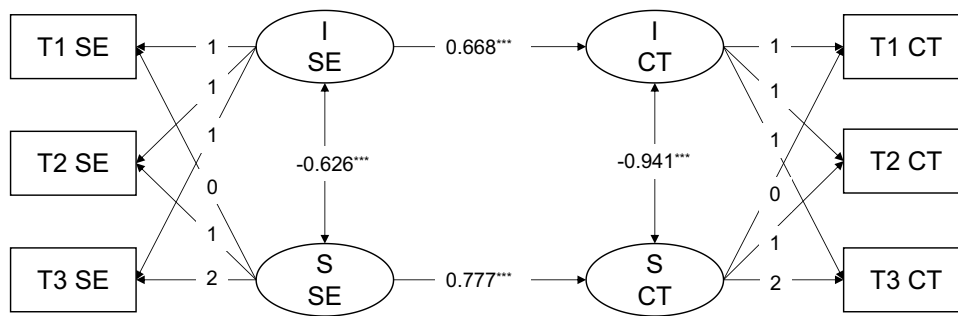
Figure 2 LGM of study engagement and critical thinking. Note: *** p<0.001. Abbreviations: LGM, latent growth model; I SE, intercept of study engagement; S SE, slope of study engagement; I CT, intercept of critical thinking; S CT, slope of critical thinking; T1, T2, T3, Time 1, Time 2, Time 3.
