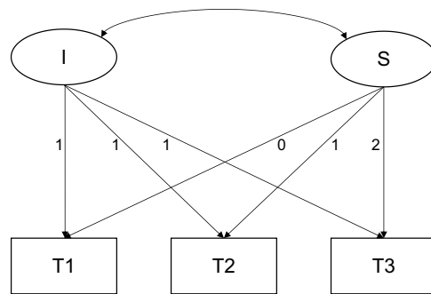
Figure 1 LGM with unconditional variables of study engagement or critical thinking. Abbreviations: LGM, latent growth model; I, intercept; S, slope; T1, T2, T3, Time 1, Time 2, Time 3.
