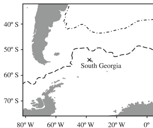
Figure 1. Location of Bird Island, South Georgia (cross), in relation to the APF (dashed line) and STF (dot-dash line).
