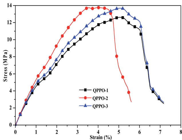
Fig. 9 Stress-strain behavior for QPPOs membranes.
