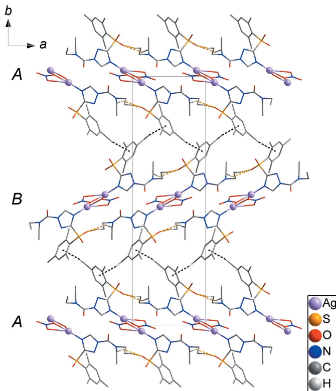
Figure 4 The packing diagram showing the three-dimensional network structure formed by C–H...O hydrogen bonds and C–H...π interactions (shown as yellow and black dashed lines, respectively).
