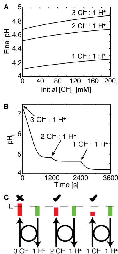
Figure 8. The influence of CIC-7 antiporter stoichiometry on acidification. (A) Steady-state pH_L values over a range of initial [Cl^-]_L values are plotted for a model lysosome containing 300 V-ATPases, P_{H^+} of 6 \times 10^{-5} cm/s, and 5,000 CIC-7 antiporters of varying stoichiometry. A putative antiporter with a 1:1 stoichiometric ratio gives rise to the greatest acidification. (B) Time-dependent change in pH_L was calculated, starting with the stoichiometry of 3 Cl^- :1 H^+ . After the pH reached steady state, the stoichiometric ratio was changed to 2 Cl^- :1 H^+ and then to 1 Cl^- :1 H^+ . After each change, the system achieved a lower pH_L . (C) At a given pH gradient, the antiporter has a fixed amount of energy (E) provided by the proton movement during one cycle (green bars). If the transport is 3:1, the energy required for Cl^- movement against their gradient (red bars) is greater than the energy provided by proton movement, and transport will not happen (indicated by the X). When the ratio is 2:1, the antiporter is close to stalling, but there is just enough energy to complete the cycle and pump Cl^- into the lumen, which will subsequently allow further acidification by the V-ATPase (check mark). When the ratio is 1:1, there is ample energy to allow Cl^- transport into the lumen (check mark). All other parameter values are given in Table 1.
