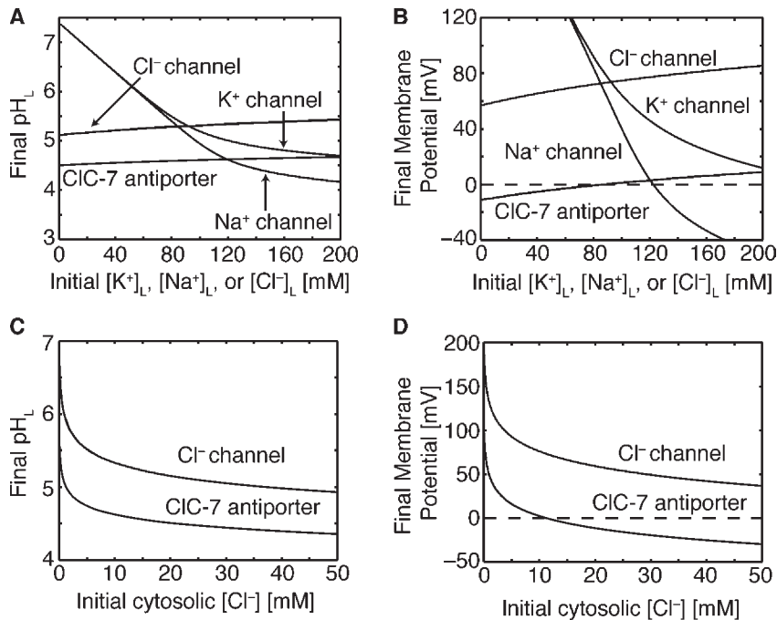
Figure 4. Steady-state pH L in the presence of the V-ATPase proton pump. (A) Steady-state pH L as a function of initial luminal concentration for four different counterion flows: ClC-7 antiporter, Cl - , K + , or Na + channel. For each curve, the initial concentration of the ion being transported was varied from 1 to 200 mM. Thus, for simulations including Cl - channels, the initial [Cl - ] L was varied from 1 to 200 mM, and the steady-state pH L was determined for each concentration. (B) The steady-state membrane potentials for the simulations in A. (C) Steady-state pH L as a function of cytosolic Cl - concentration for models containing either Cl - channels or ClC-7 antiporters. (D) The steady-state membrane potentials for the simulations in C. All simulations included P_{H^+} of 6 \times 10^{-5} cm/s and 300 V-ATPases. Simulations with ClC-7 antiporters included 5,000 transporters, and the model lysosome was spherical with a diameter of 0.68 \mu m (Van Dyke, 1993). In all simulations, the initial luminal concentrations of ions were equal to typical extracellular values, except for the concentrations being explicitly varied along the x axes. All other parameter values are given in Table 1.
