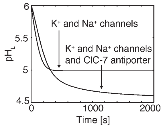
Figure 5. Dynamics of lysosomal acidification for two different counterion pathway models. The top curve is from a model containing only K + and Na + channels, and the bottom curve is from a model that has both cation channels in addition to ClC-7 antiporters. The initial conditions were set to [K + ] L = 50 mM, [Na + ] L = 20 mM, [Cl - ] L = 1 mM, and pH L 6.0 as reported by Steinberg et al. (2010). For these values, cation channels alone can achieve a pH L of 5.0, but the addition of ClC-7 lowers the pH another 1/2 unit. Both simulations included P_{H^+} of 6 \times 10^{-5} cm/s and 300 V-ATPases. The simulation with ClC-7 antiporters included 300 transporters. The buffering capacity was 40 mM/pH, and all other parameter values are given in Table 1.
