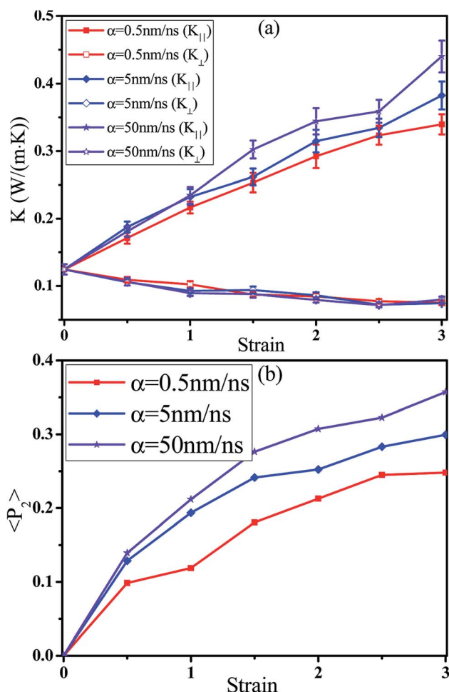
Fig. 5 Change of the thermal conductivities (a) K_{||} ( \text{W m}^{-1} \text{ K}^{-1} ) parallel to tensile direction, K_{\perp} ( \text{W m}^{-1} \text{ K}^{-1} ) perpendicular to tensile direction, and (b) the orientation degree \langle P_2 \rangle of backbone bonds with the strain for different tensile rates \alpha . ( T = 300 \text{ K} , composition ratio of styrene = 23%.)
