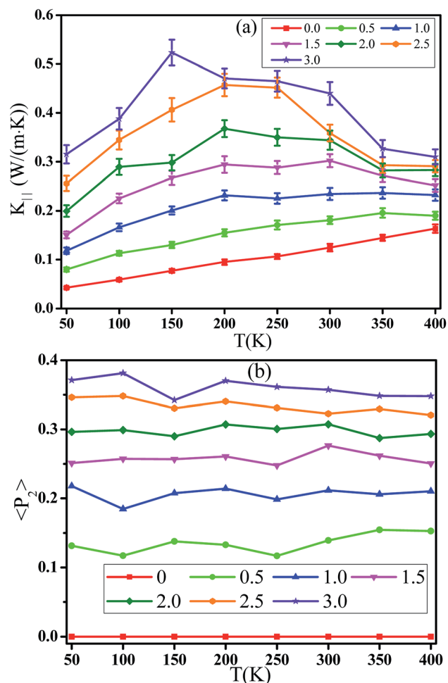
Fig. 9 Change of the (a) thermal conductivities K_{||} ( \text{W m}^{-1} \text{K}^{-1} ) parallel to tensile direction and (b) the orientation degree \langle P_2 \rangle of backbone bonds with the temperature ( T ) for different strains. (Composition ratio of styrene = 23%, \alpha = 50 nm ns ^{-1} .)
