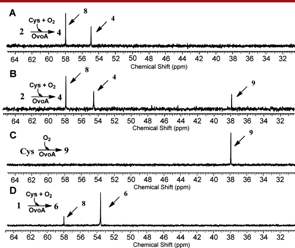
Figure 2. ^{13}\text{C} NMR analyses of OvoA reactions. (A) Formation of compound 4 and cysteine sulfinic acid 8 when hercynine and cysteine were the substrates. (B) Oxidation of cysteine to cystine in reaction A after all hercynine was consumed. (C) Formation of cystine (9) when cysteine was the only substrate. (D) Formation of compound 6 and cysteine sulfinic acid (8) when histidine and cysteine were the substrates.
