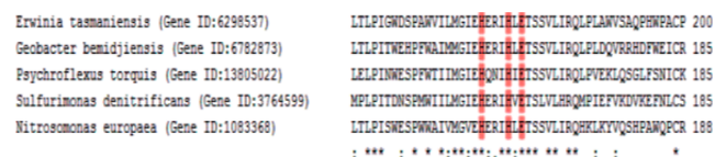
Figure 3. Sequence alignment of OvoA enzymes from a few species. Mononuclear non-heme iron ligands (2-His-1-carboxylate facial triad) are colored in red.
