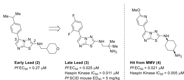
Figure 1. Early and late lead 5-aryl-2-amino-ITD antiplasmodium compounds discovered by Novartis and 5-aryl-2-amino-ITD hit disclosed by MMV.
