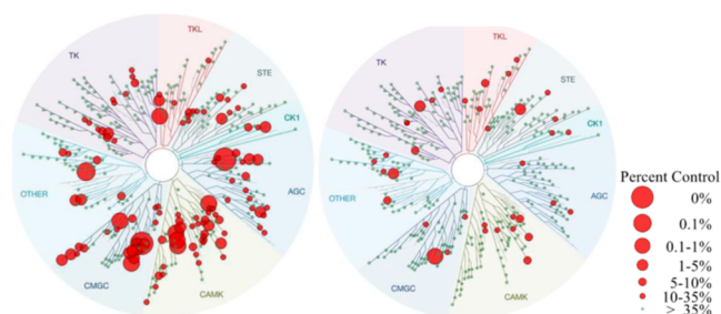
Figure 6. High-concentration (10 μM) human kinase screen of 3 (left) and INE963 (1) (right).
