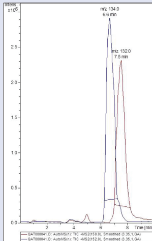
Figure 1: Mass spectroscopy chromatogram of cathinone and cathine from Khat extract. Mass spectroscopy/mass spectroscopy chromatogram of cathinone at 7.5 min m/z 150 ( \Delta 132) and cathine, at 6.6 min m/z 152 ( \Delta 134)
