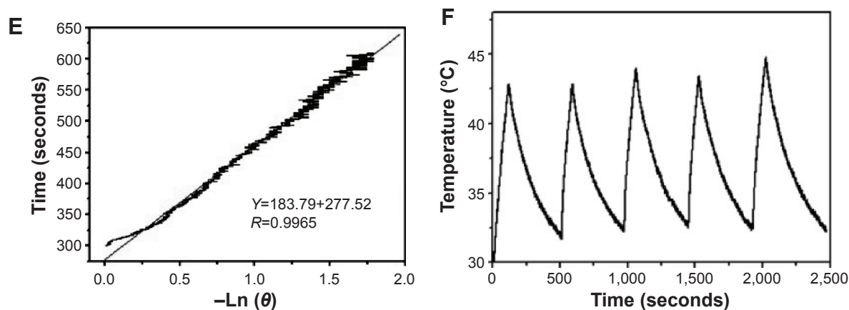
Figure 4 Photothermal conversion properties of UCNPs-PANPs.
