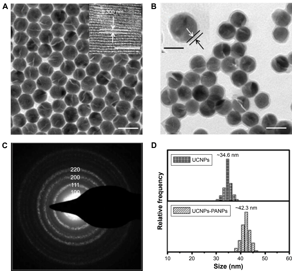
Figure 1 The morphology and size distribution of UCNPs-PANPs. Notes: TEM image of UCNPs (A) and UCNPs-PANPs (B). Scale bar: 50 nm. Inset (A): an HR-TEM image of a UCNP. Arrows indicate the distance of the lattice. (Scale bar: 5 nm) and inset (B) a UCNP-PANP. Arrows indicates thickness of the shell (Scale bar: 30 nm). (C) SAED pattern of UCNPs. (D) The particle size distribution of UCNPs and UCNPs-PANPs. The average size of UCNPs and UCNPs-PANPs is ~34.6 nm and ~42.3 nm, respectively. Abbreviations: HR-TEM, high-resolution transmission electron microscopy; SAED, selected area electron diffraction; UCNPs, upconversion nanoparticles; UCNPs-PANPs, polyaniline-coated UCNPs.
