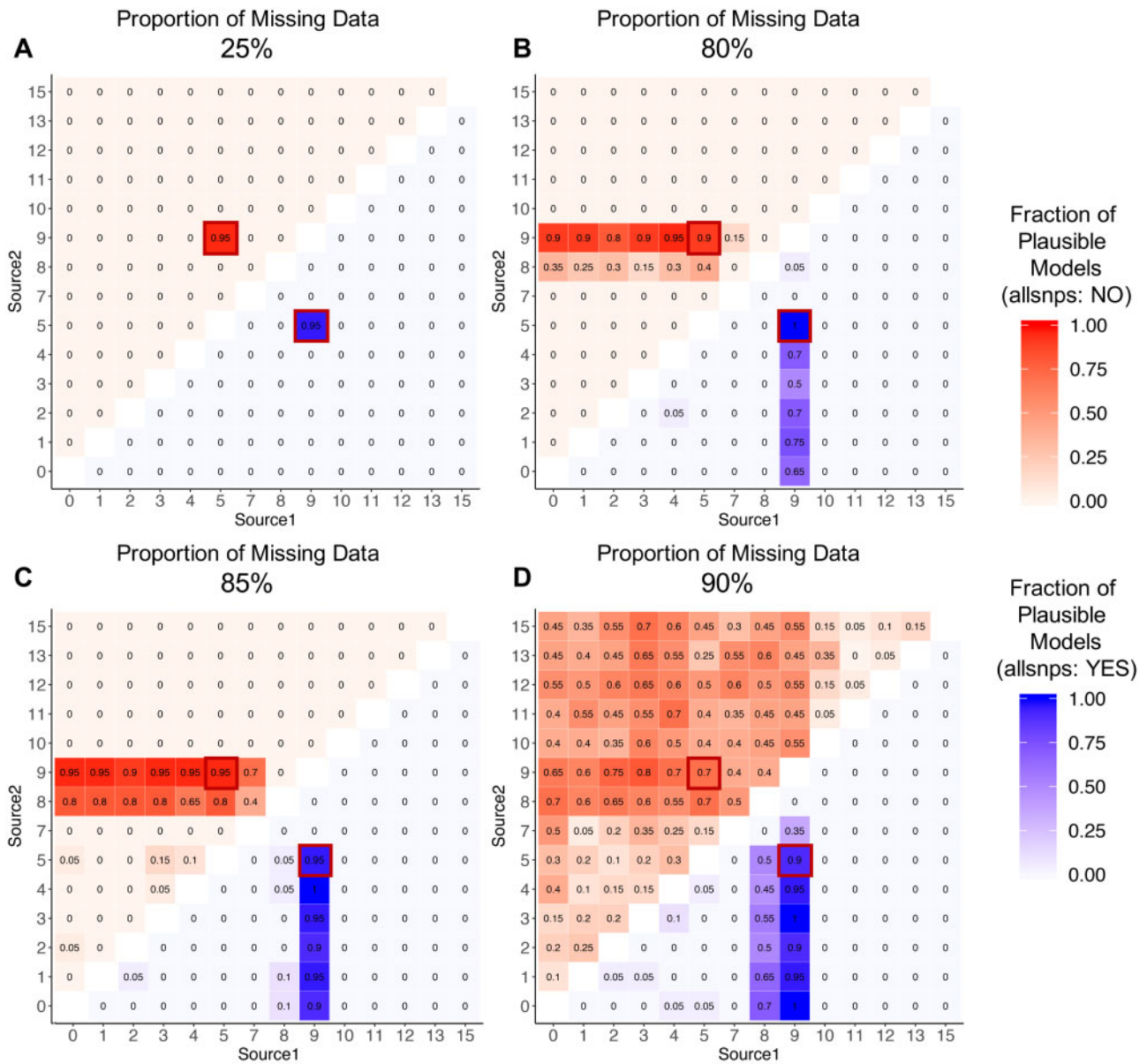
Figure 5 Effect of the allsnps parameter on qpAdm model selection. Heatmaps showing the proportion of replicates in which the two-way admixture model generated using each combination of possible source populations is deemed plausible by qpAdm (i.e. yielded a P-value > 0.05 and admixture proportion estimates between 0 and 1) on SNP data using the “allsnps: yes” (blue; lower right triangle) and “allsnps: no” parameters (red; upper left triangle), on data with (A) 25% (B) 80% (C) 85%, or (D) 90% missing data. The proportion of replicates deemed plausible is indicated by the color (darker shades indicate a higher proportion) and is written inside each square of the heatmap. The optimal admixture model for each of the approaches are highlighted in red.
