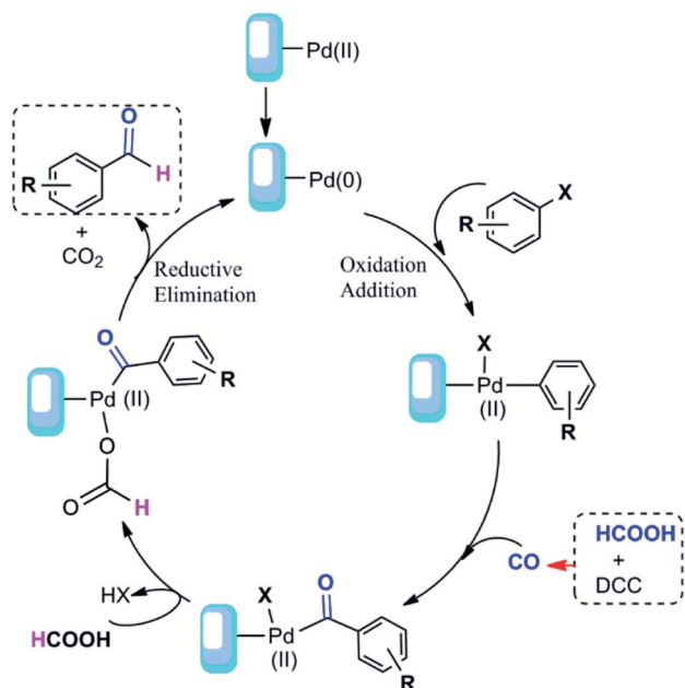
Scheme 4 Proposed mechanism of the carbonylation reaction.
