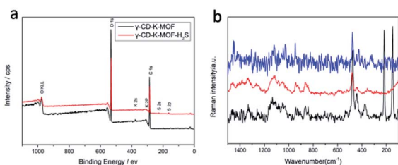
Fig. 1 (a) XPS spectra of \gamma -CD-K-MOF and \gamma -CD-K-MOF-H 2 S (b) Raman spectra of the \gamma -CD-K-MOF (red), \gamma -CD-K-MOF-H 2 S (black) and \gamma -CD-K-MOF-H 2 S heated under vacuum at 130 °C for 7 h (blue).
