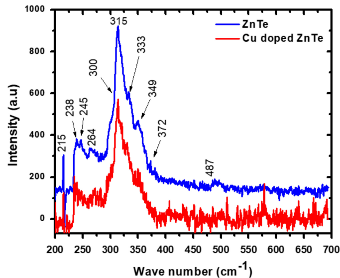
Figure 3. Room temperature Raman spectra of un-doped ZnTe and Cu-doped ZnTe thin film samples.
