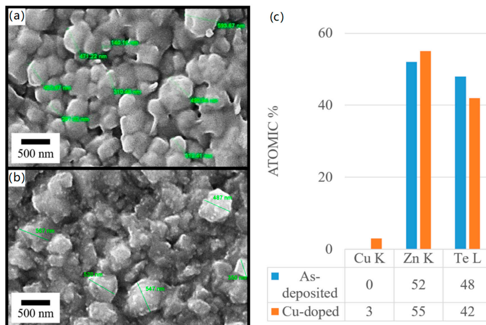
Figure 4. Scanning Electron Micrographs of (a) un-doped and (b) Cu-doped ZnTe thin film samples with (c) EDX analyses of un-doped and Cu-doped ZnTe thin film samples shows a Cu content of 3 at.% in Cu-doped samples.
