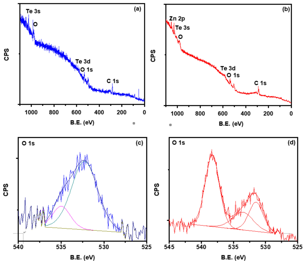
Figure 6. XPS Survey scan of (a) un-doped and (b) Cu-doped ZnTe thin film samples. De-convoluted XPS analysis of Oxygen-1s for (c) un-doped and (d) Cu-doped ZnTe thin film samples.
