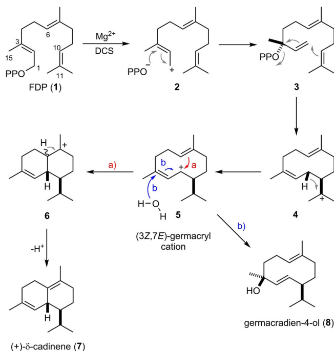
Scheme 1. Catalytic mechanisms of the DCS (pathway a) and GdoS (pathway b) catalysed conversions of 1 to 7 and germacradien-4-ol ( 8 ).
