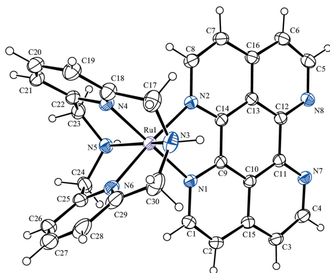
Figure 1 The molecular structure of [Ru(L-N_4H_2)tape]^{2+} in [Ru(L-N_4H_2)tape](PF_6)_2 \cdot 1.422CH_3CN] with the atomic numbering scheme and 30% probability displacement ellipsoids. Anions and solvent molecules are omitted for clarity.
