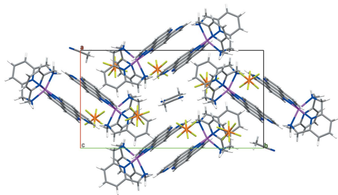
Figure 3 A packing diagram of the title compound is displayed along the c axis, illustrating the herringbone-type motif formed by two [Ru(L-N 4 H 2 )-tape] 2+ dimers. The disordered minor atoms are omitted for clarity.
