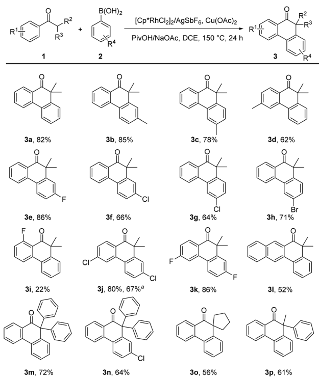
Scheme 2 Scope of substrates. Reaction conditions: 1 (0.2 mmol), 2 (0.6 mmol), [\text{Cp}^*\text{RhCl}_2]_2 (5.0 mol%), \text{AgSbF}_6 (20 mol%), \text{Cu}(\text{OAc})_2 (2.0 equiv.), PivOH (1.2 equiv.), NaOAc (0.2 equiv.) and DCE (1.0 mL) at 150 °C for 24 h under \text{N}_2 . Isolated yields. a 1.0 mmol scale.
