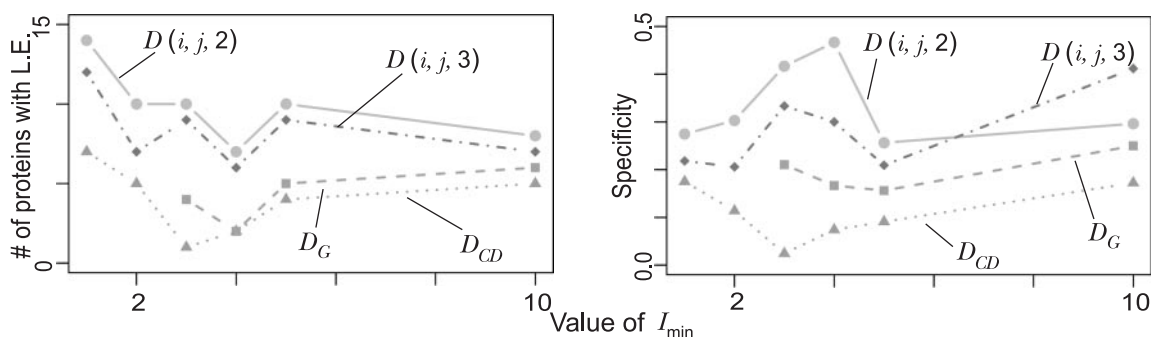
Figure 2. Comparison by other distance functions. P_B \leq 0.001 , O_{\min} = 3 and P_{mw} \leq 0.05 are used. The number of predictions with literature evidence is relevant to sensitivity of each condition. Specificity = No. of predictions with literature evidence/No. of predictions. As for D_G and D_{CD} , mean is used instead of median as the central tendency. There are proteins whose distances are not defined in using D_G with I_{\min} = 1 or 2. Thus, results on D_G with I_{\min} = 1 and 2 are omitted.
