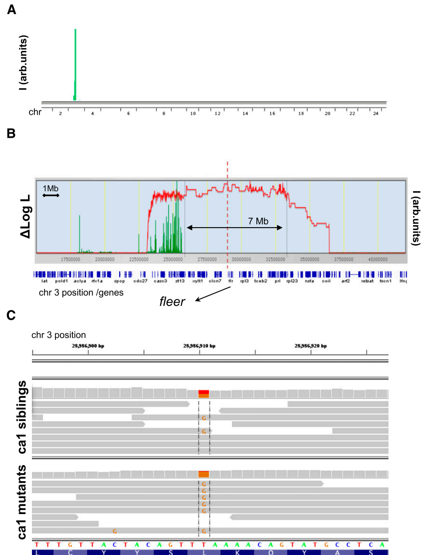
Figure 3. Mapping of ca1 . (A) Homozygosity scoring reveals a single peak on chromosome 3. (B) Log likelihood analysis (red line) returns a ~7-Mb interval for the presumptive mutation, while the homozygosity score (green graph) misses the mutation region due to very low SNP frequency in some areas of the interval. (C) Sequencing of exon 6 of the flr gene reveals a premature stop codon.
