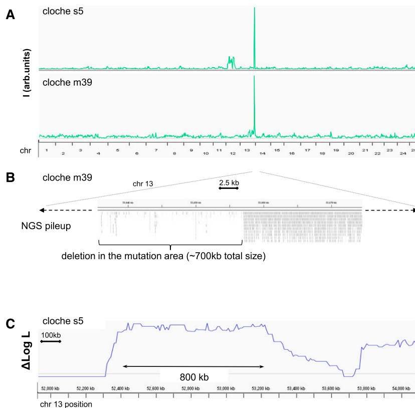
Figure 2. Mapping of two alleles of the cloche mutant. (A) Homozygosity scoring of the clo s5 and clo m39 alleles reveals corresponding overlapping peaks on chromosome 13, where the mutation has been previously mapped. (B) Sequence pileup of the clo m39 allele confirms the previously established deletion and reveals the boundaries of the deletion interval. (C) Log likelihood scoring of the clo s5 alleles achieves a higher resolution of the mutation region with a narrower interval than the homozygosity scoring method.
