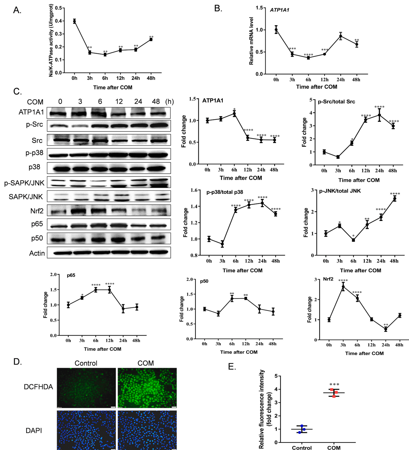
Fig. 2. COM exposure to HK2 cells activated the ATP1A1/Src/ROS/MAPKs/NF-κB signaling pathway. HK2 cells were exposed to 100 µg/mL COM for 0, 3, 6, 12, 24, and 48 h. Each experiment was independently repeated at least thrice. (A) The activity of NKA in HK2 cells decreased after COM stimulation. The data were expressed as the mean ± SD (n = 5). ** p < 0.01 vs. levels at 0 h. (B) COM exposure to HK2 cells inhibited the mRNA level of ATP1A1 . The data were expressed as the mean ± SEM (n = 3). ** p < 0.01; *** p < 0.001; **** p < 0.0001 vs. levels at 0 h. (C) Western blotting analysis for the expressions of ATP1A1, p65, p50, Nrf2, and the phosphorylation of Src, p38, and JNK after COM exposure. The relative levels of proteins were calculated as a fold change relative to the level at 0 h. The data were expressed as the mean ± SD (n = 3). * p < 0.05; ** p < 0.01; **** p < 0.0001 vs. the level at 0 h. (D–E) HK2 cells were exposed to 100 µg/mL COM for 24 h. Intracellular ROS was detected with a green fluorescent probe DCFHDA. The nuclei were stained with DAPI (blue). Scale bar = 50 µm. The relative fluorescence intensity was calculated as the fold change relative to the control group. The data were expressed as the mean ± SD (n = 3). *** p < 0.001 vs. the control. (For interpretation of the references to color in this figure legend, the reader is referred to the Web version of this article.)
