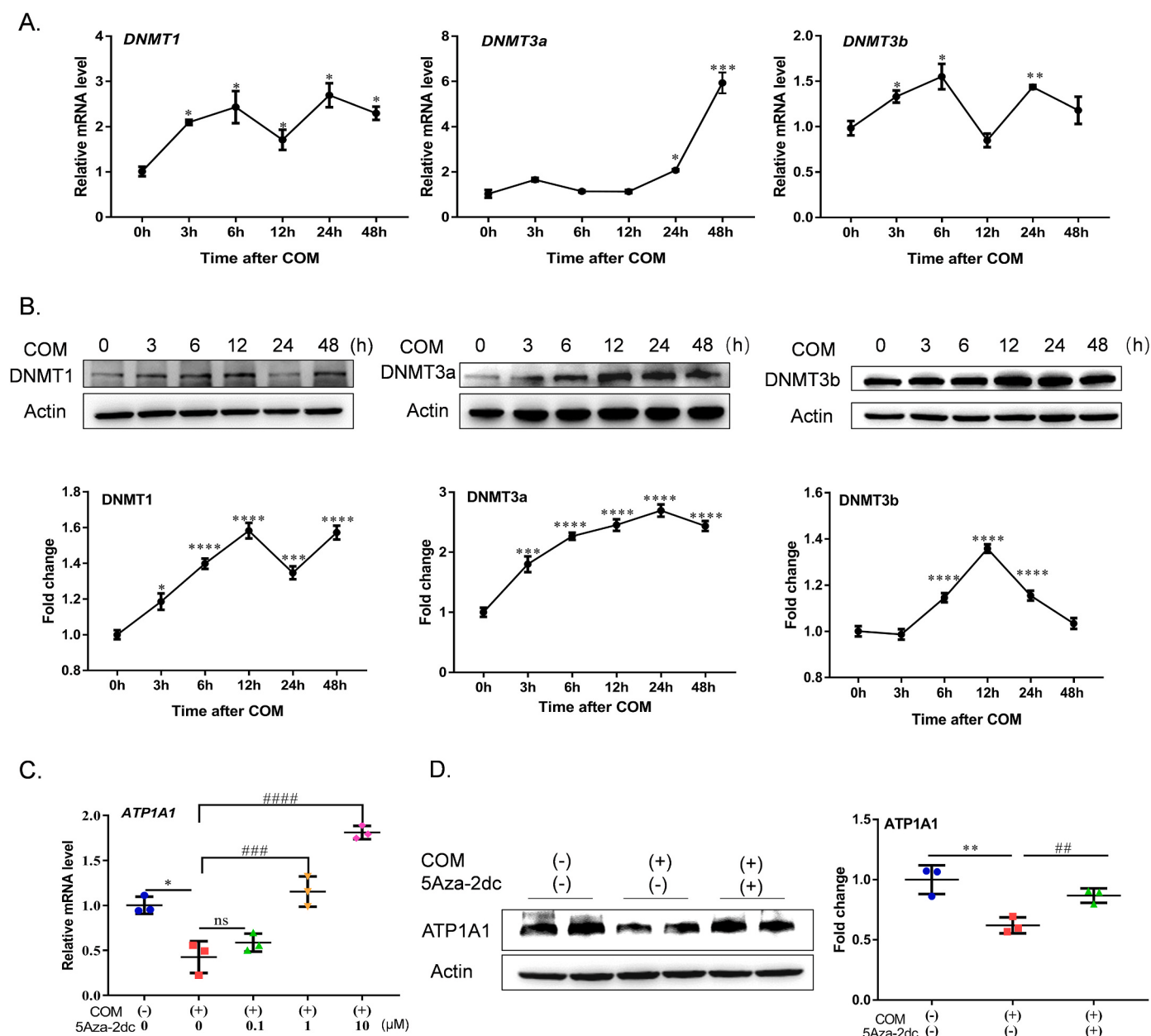
Fig. 6. DNA methylation participated in the downregulation of ATP1A1 induced by COM. (A) After exposing 100 \mu g/mL COM to HK2 cells, the mRNA levels of DNMT1 , DNMT3a , and DNMT3b , were measured by qRT-PCR. The values were expressed as the mean \pm SEM ( n = 4 ). ^*p < 0.05 ; ^{**}p < 0.01 ; ^{***}p < 0.001 ; vs. the levels at 0h. (B) The protein levels of DNMT1, DNMT3a, and DNMT3b were determined by Western blotting. The relative expression level was expressed as a fold change relative to the level at 0 h. Each experiment was repeated thrice, independently. The values were expressed as the mean \pm SEM ( n = 3 ). ^*p < 0.05 ; ^{**}p < 0.01 ; ^{***}p < 0.001 ; ^{****}p < 0.0001 vs. the levels at 0 h. (C) The ATP1A1 mRNA level was detected after pretreatment with 5Aza-2dc, a specific inhibitor of DNA methyltransferase, at the concentration of 0.1–10 \mu M. The values were expressed as the mean \pm SEM ( n = 3 ). ^*p < 0.05 vs. COM (-); ^{###}p < 0.001 ; ^{####}p < 0.0001 vs. only COM (+). (D) The protein level of ATP1A1 was examined by Western blotting after pretreatment with 10 \mu M 5Aza-2dc. Three independent experiments were performed and the values were expressed as the mean \pm SD ( n = 3 ). ^{**}p < 0.01 vs. COM (-). ^{##}p < 0.01 vs. only COM (+).
