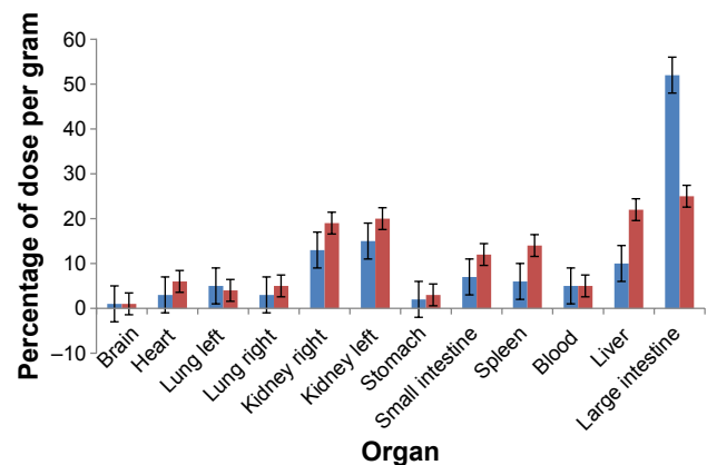
Figure 6 Biodistribution of PLA/PVA/MMT/trastuzumab nanoparticle labeled with 99m Tc (red) compared with trastuzumab (free drug) labeled with 99m Tc (blue).
