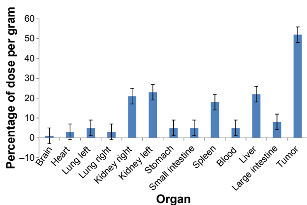
Figure 7 Biodistribution of the PLA/PVA/MMT/trastuzumab nanoparticles labeled with ^{99m}\text{Tc} in female Balb/C nude mice induced with breast cancer in the flank. Abbreviations: MMT, montmorillonite; PLA, polylactic acid; PVA, polyvinyl alcohol.
