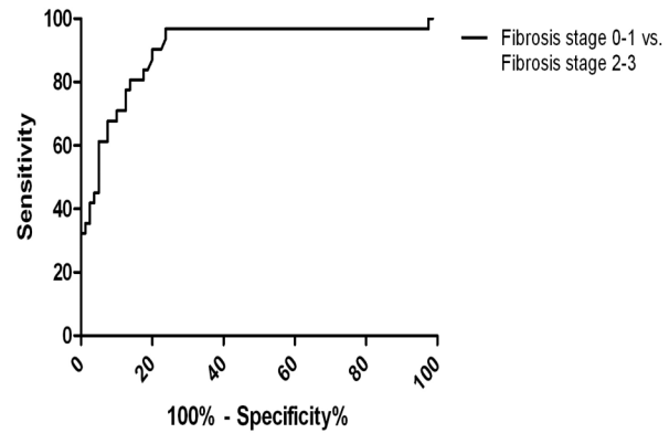
Fig. 3. ROC curves for 13 C-methionine breath test outcome parameter cumulative percentage recovery after 90 min test time (cPDR 1.5h ) in patients with non-alcoholic fatty liver (NAFL). A: for differentiation of non-NASH (steatosis and borderline-diagnosis) from NASH in the total cohort (solid line) and a subgroup of patients (n = 92) with mild (F0-1) fibrosis (dashed line). B: for differentiation of non-significant (F0-1) from advanced (F2-3) fibrosis in 99 patients with borderline diagnosis or definite NASH.
