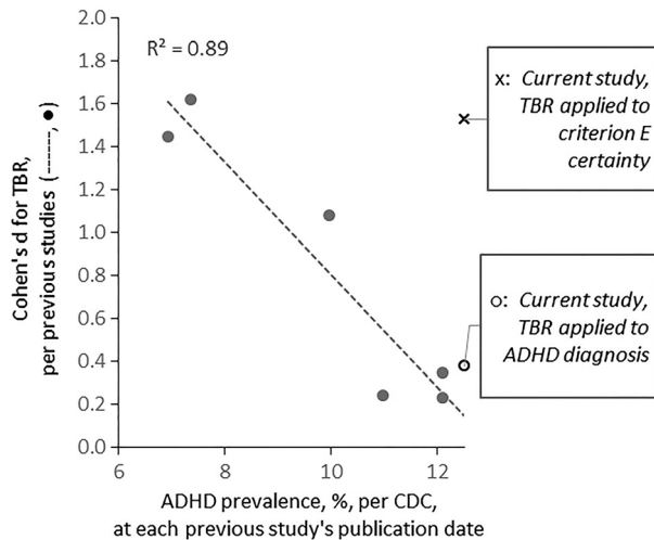
Figure 1. Cohen's d values (for each of six previous studies that were included in a recent meta-analysis by Arns et al. 2013 to represent ages 6–18 years) have been plotted relative to ADHD prevalence (per CDC estimates applied to each study's publication date (CDC, 2014; Visser et al. 2014)) (●). Linear fit (-----) shows an inverse relationship ( R^2 , 0.89). In the current study, applying TBR to ADHD diagnosis per an individual clinician (o) has reduced statistical power as predicted by the trend; however, applying TBR to improve certainty of criterion E per a Multidisciplinary Team (x) restores statistical power to prior levels.
