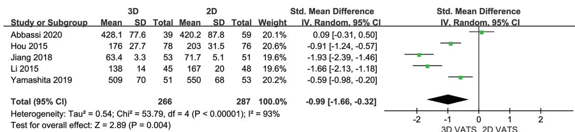
Figure 5 Forest plot of the role of SMD and its 95% CI of operation time between 3D and 2D VATS group. SMD, standardized mean difference; CI, confidence interval; VATS, video-assisted thoracic surgery.
