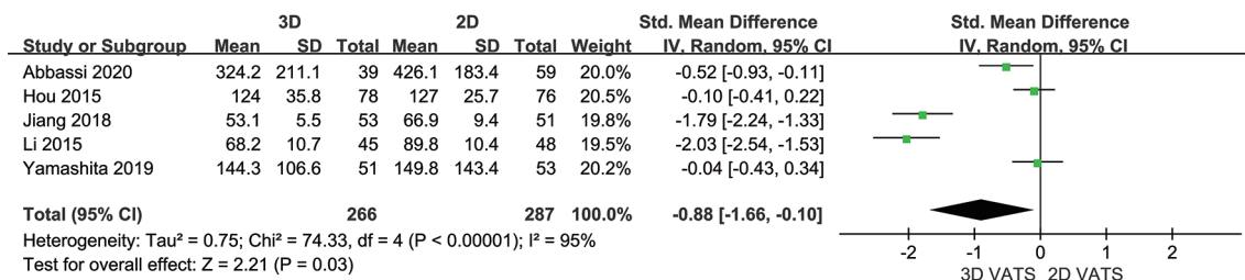
Figure 6 Forest plot of the role of SMD and its 95% CI of operative blood loss between 3D and 2D VATS group. SMD, standardized mean difference; CI, confidence interval; VATS, video-assisted thoracic surgery.
