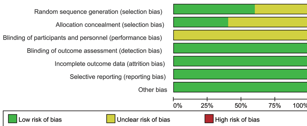
Figure 2 Risk of bias graph according to the Cochrane collaboration’s tool.
