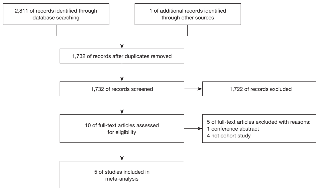
Figure 4 Preferred reporting items for meta-analyses flow chart of literature selection.
