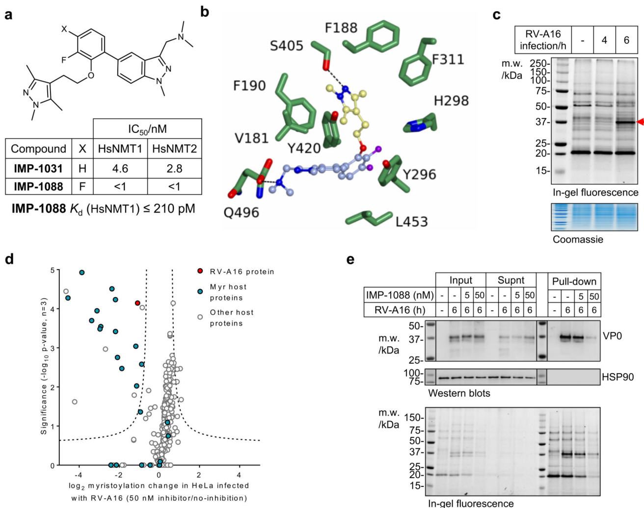
Figure 3. Potent inhibitors of human N -myristoyltransferases inhibit rhinovirus myristoylation in infected cells.
