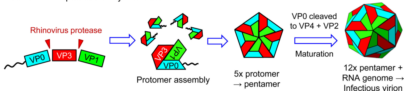
Figure 1. Proposed pathway for generation of infectious rhinovirus particles in an infected host cell.
