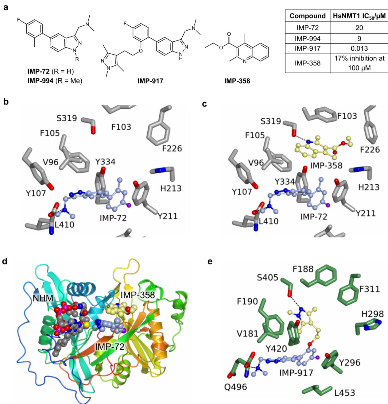
Figure 2. Structure-guided discovery of potent human N -myristoyltransferase inhibitors.
