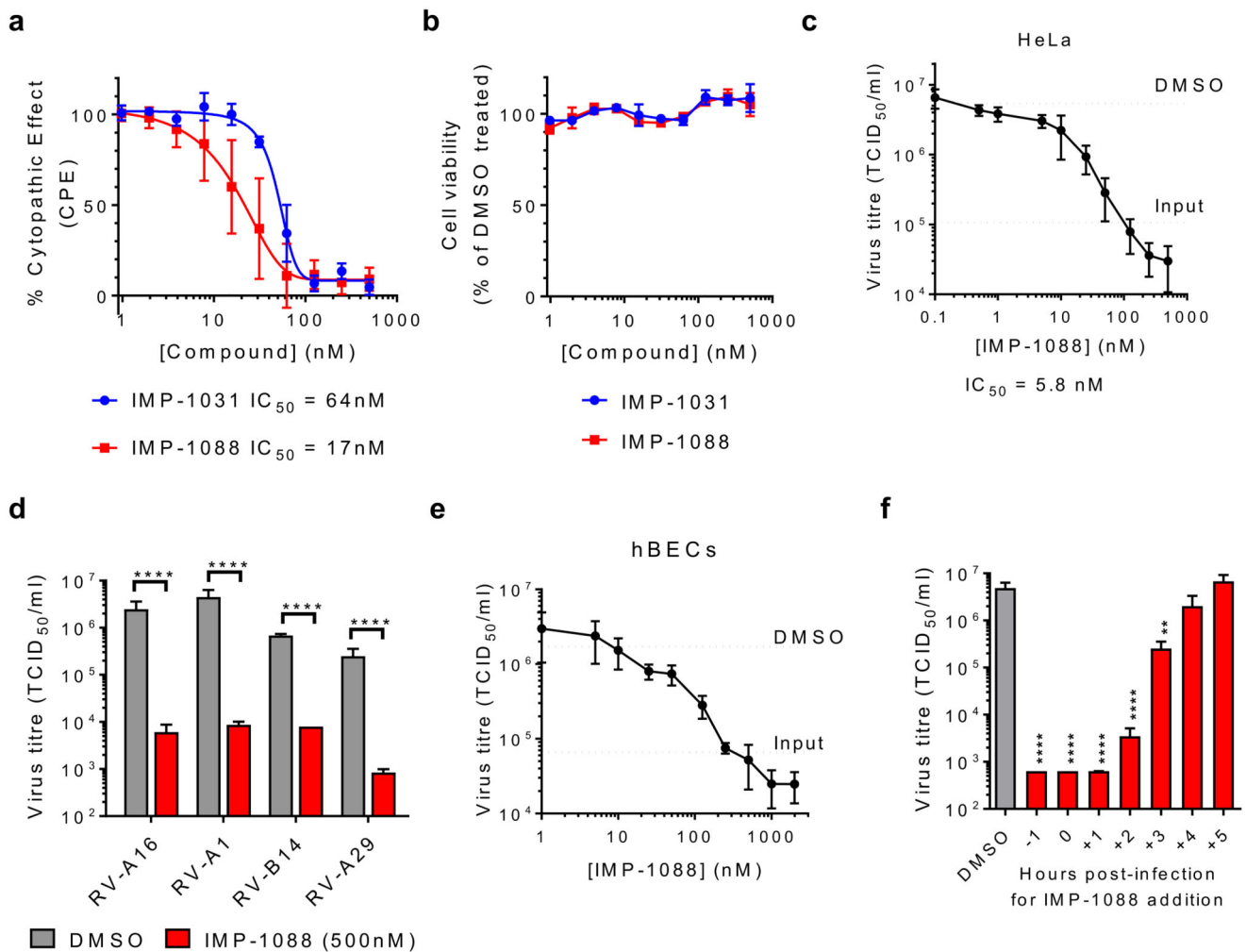
Figure 4. Novel human N -myristoyltransferase inhibitors potently and efficiently block rhinovirus replication without cytotoxicity.
