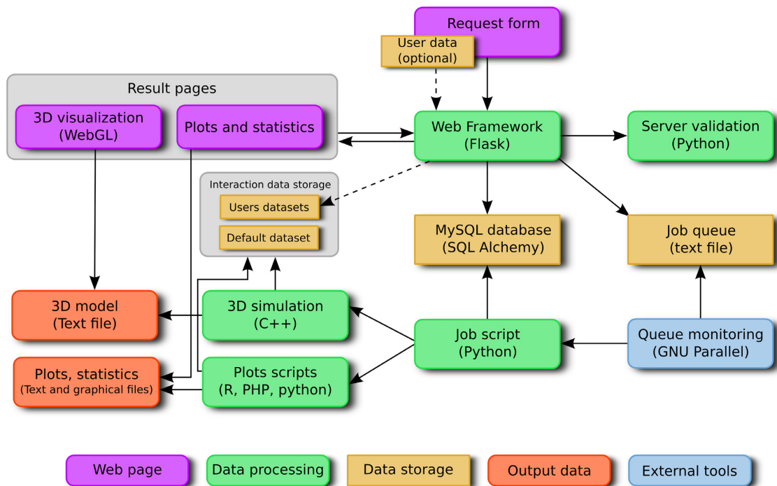
Figure 1. Webservice architecture. The central role is played by a Flask-based server which accepts the requests, stores them in the database and adds them to the job queue. GNU Parallel monitors the queue and runs the jobs as soon as there are computational resources available. Each job consists of a number of external scripts executed sequentially.
