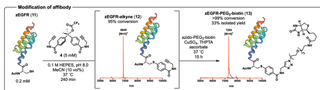
Scheme 4 Arylation of zEGFR affibody 11 with 4 to afford the intermediate 12 , which was converted to biotin conjugate 13 in one-pot using the CuAAC reaction. Structure of zEGFR from PDB (ID: 2KZI).
