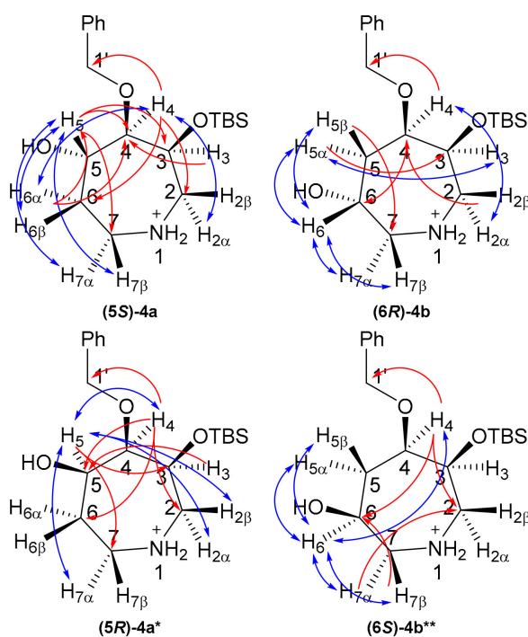
Figure 1. 2D-NMR correlations for azepanols (5S)-4a and (6R)-4b. Red, HMBC; blue, NOESY.
