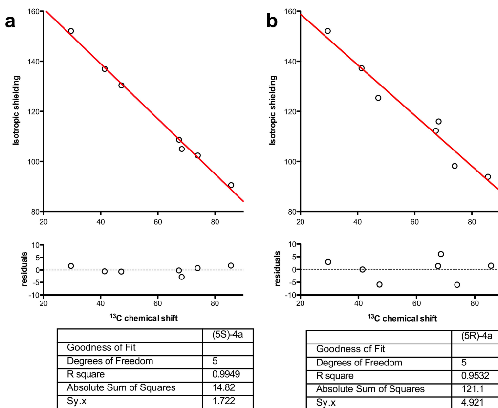
Figure 2. Non-linear regression fitted to a straight line of chemical shifts against calculated isotropic shielding (DFT//B3-LYP/TZVPP) for (a) (5S)- 4a and (b) (5R)- 4a with residuals and goodness-of-fit values.
