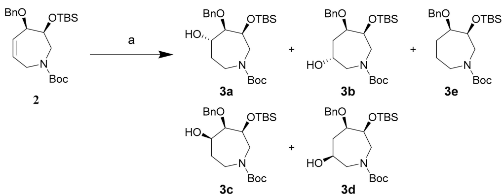
Scheme 4. Reagent and catalyst screen for the hydroboration of 2 . Conditions (a) (i) \text{BHR}_2 , see Table 2, THF; (ii) \text{NaOH} , \text{H}_2\text{O}_2 , EtOH, 80 °C, 1 h, 99%.
