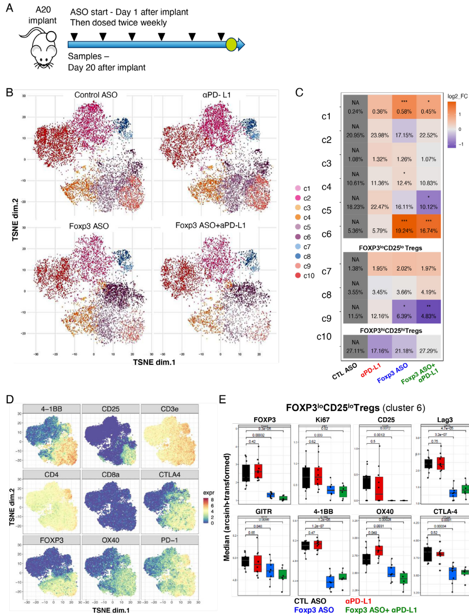
Figure 6 FOXP3 ASOs reprogram Treg effector cell phenotype in vivo in combination with \alpha PD-L1 immune checkpoint blockade. (A) Mice were treated with ASO (50 mg/kg BIW) and \alpha PD-L1 (10 mg/kg BIW) alone or in combination from day 1 post A20 tumor-implantation. N=14 per group. Tumors were analyzed by mass cytometry at day 20 after implantation. (B) t-SNE analysis of tumor-infiltrating CD4 + T cells. (C) Relative changes of CD4 + T cell clusters compared with control group. (D) Expression map of T cells and Tregs markers. (E) Quantification of Treg activation expression markers. Error bars are SD. *, p \leq 0.05 ; **, p \leq 0.01 ; ***, p \leq 0.001 ; ****, p \leq 0.0001 by one-way analysis of variance with Dunnett's post-test relative to control ASO. ASOs, antisense oligonucleotides; BIW, two times per week; t-SNE, t-distributed stochastic neighbor embedding; PD-L1, programmed cell death ligand 1; Treg, Regulatory T cells.
