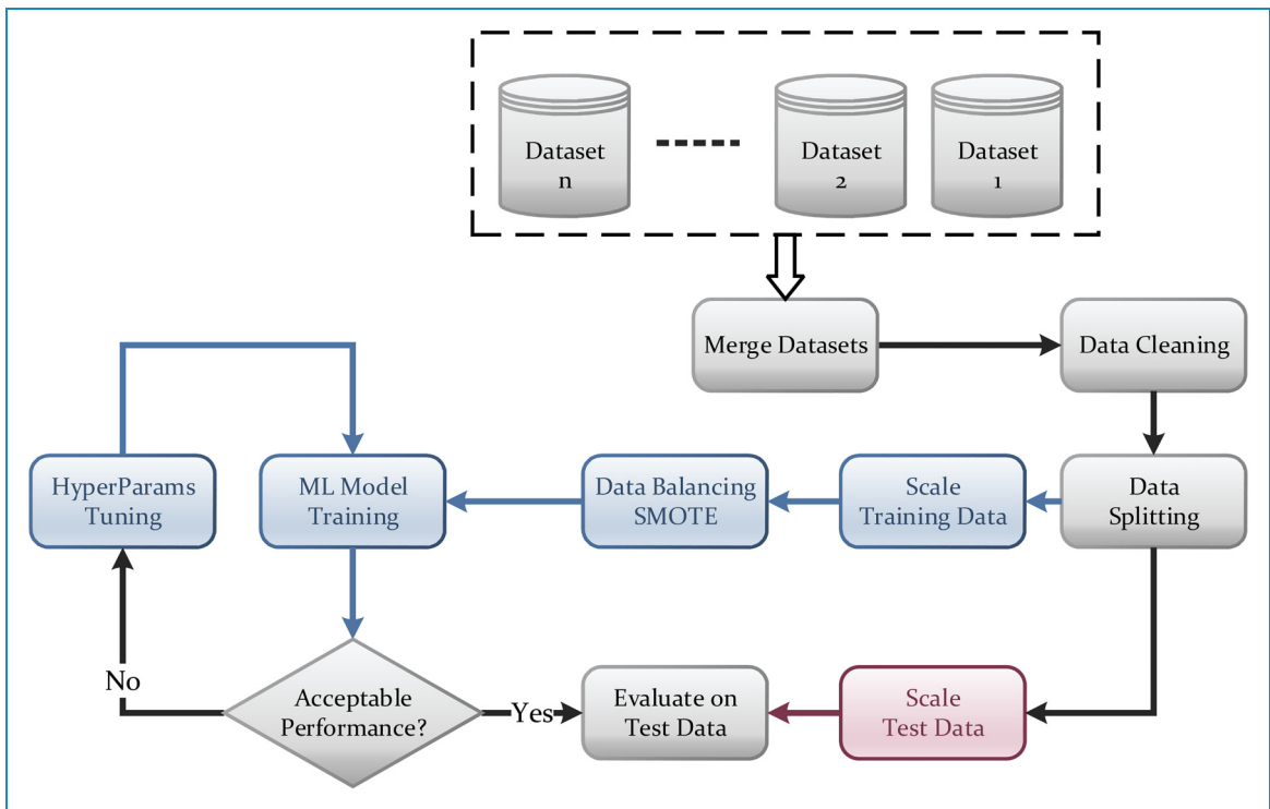
Figure 4. Data pipeline.
