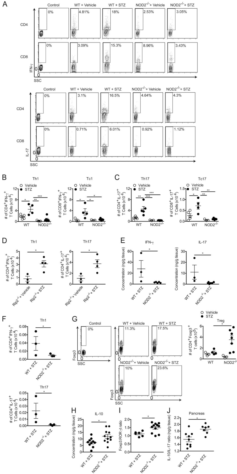
Figure 5. The NOD2 receptor is involved in the generation of Th1 and Th17 cells in vivo. Cells from the PLNs (A, B, C, D, G, and I) or pancreas (F) of WT, Rip2 -/- , or NOD2 -/- mice were harvested 15 d after vehicle or STZ administration. The frequency (A and G) and absolute numbers (B–D, F, G, and I) of CD4 + IFN- \gamma + (Th1), CD8 + IFN- \gamma + (Tc1), CD4 + IL-17 + (Th17), CD8 + IL-17 + (Tc17), and CD4 + Foxp3 + (T reg) cells and the Foxp3/ROR \gamma cell ratio were assessed by flow cytometry. The gate was set on CD3 + T cells. Alternatively, the production of IFN- \gamma and IL-17 (E), IL-10 alone (H), or the IL-10/IL-17 ratio (J) was measured in the pancreatic tissue by ELISA 15 d after the STZ injections. Data are representative of at least two independent experiments. The results are expressed as the mean \pm SEM ( n = 4 –6 mice per group). *, P \leq 0.05 ; **, P \leq 0.01 ; ***, P \leq 0.001 .
