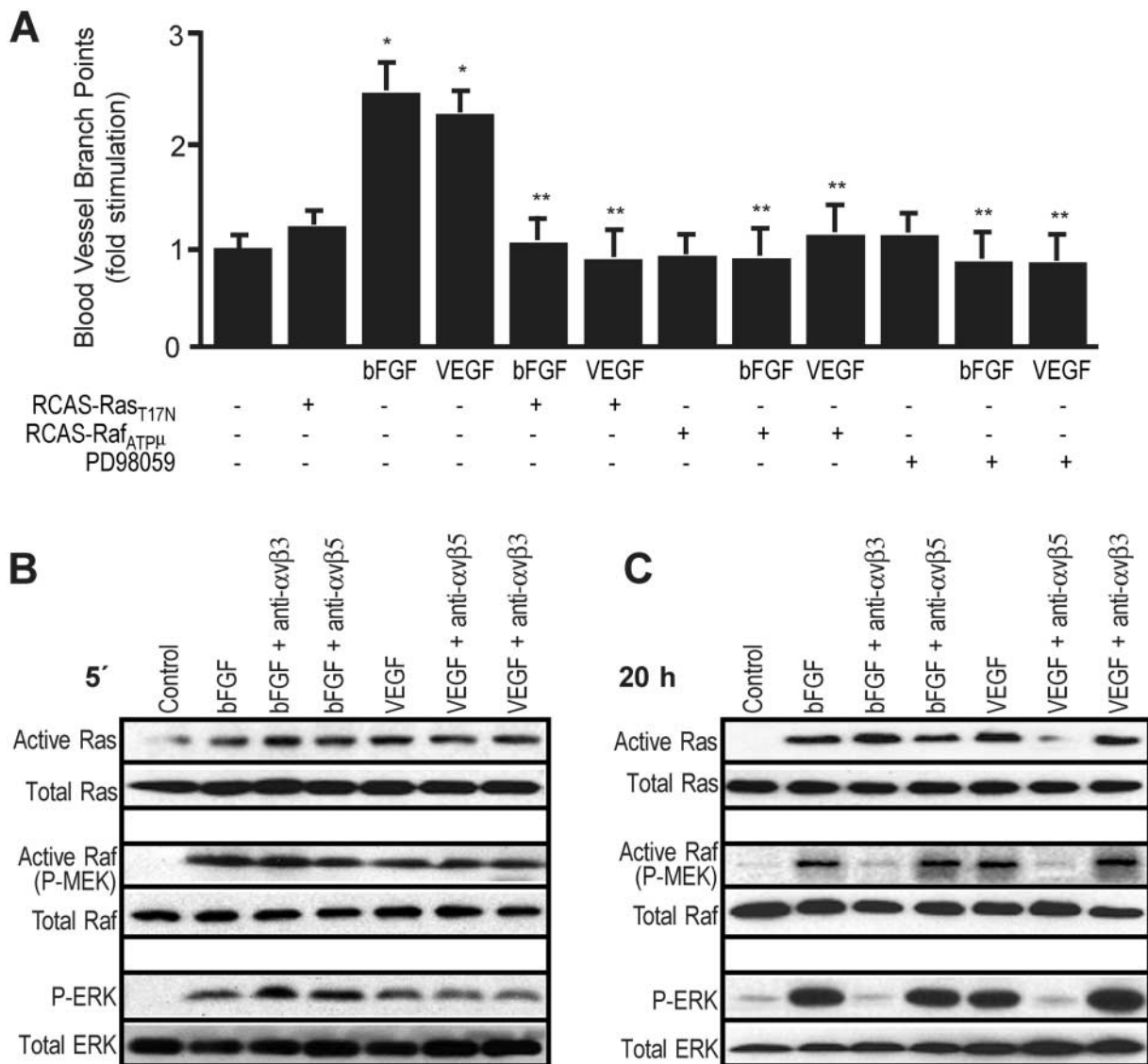
Figure 1. FGF and VEGF require and stimulate Ras, Raf, and ERK activity during angiogenesis in cooperation with integrins \alpha v \beta 3 and \alpha v \beta 5. (A) 10-d-old chick CAMs were exposed to filter paper disks saturated with RCAS-Ras T17N (inactive Ras), RCAS-Raf ATP \mu (inactive c-Raf), or PD98059 (MEK inhibitor) followed by stimulation with either 2 \mu g/ml bFGF or VEGF for 72 h. Blood vessels were enumerated by counting vessel branch points in a double-blinded manner. Each bar represents the mean \pm SEM of 24 replicates. *, P < 0.05 relative to control; **, P < 0.05 relative to treatment. (B) 10-d-old chick CAMs were exposed to filter paper disks saturated with either bFGF or VEGF for 5 min, followed by excision and detergent extraction of the tissues. 1 h before excision, the embryos were i.v. injected with 30 \mu g function-blocking antibodies selective for either integrin \alpha v \beta 3 (LM609) or \alpha v \beta 5 (P1F6). Relative Ras, c-Raf, and ERK was determined as described in Materials and methods. (C) Chick CAMs were treated as above with the exception that CAM tissue was excised 20 h after initial exposure to bFGF and VEGF.
